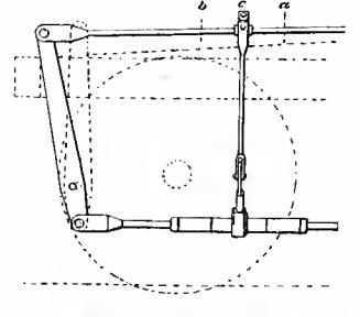
THE HINCKLEY BRAKE SLACK ADJUSTER EQUIPMENT D.
